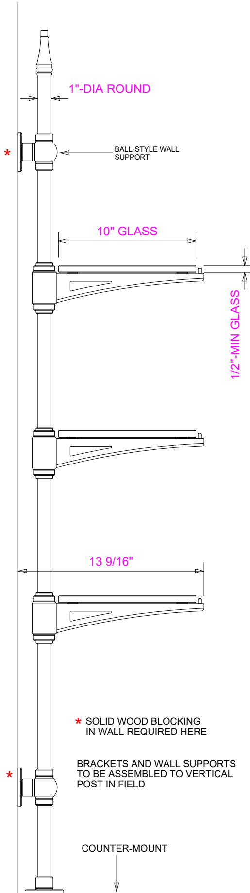
SIDE VIEW
