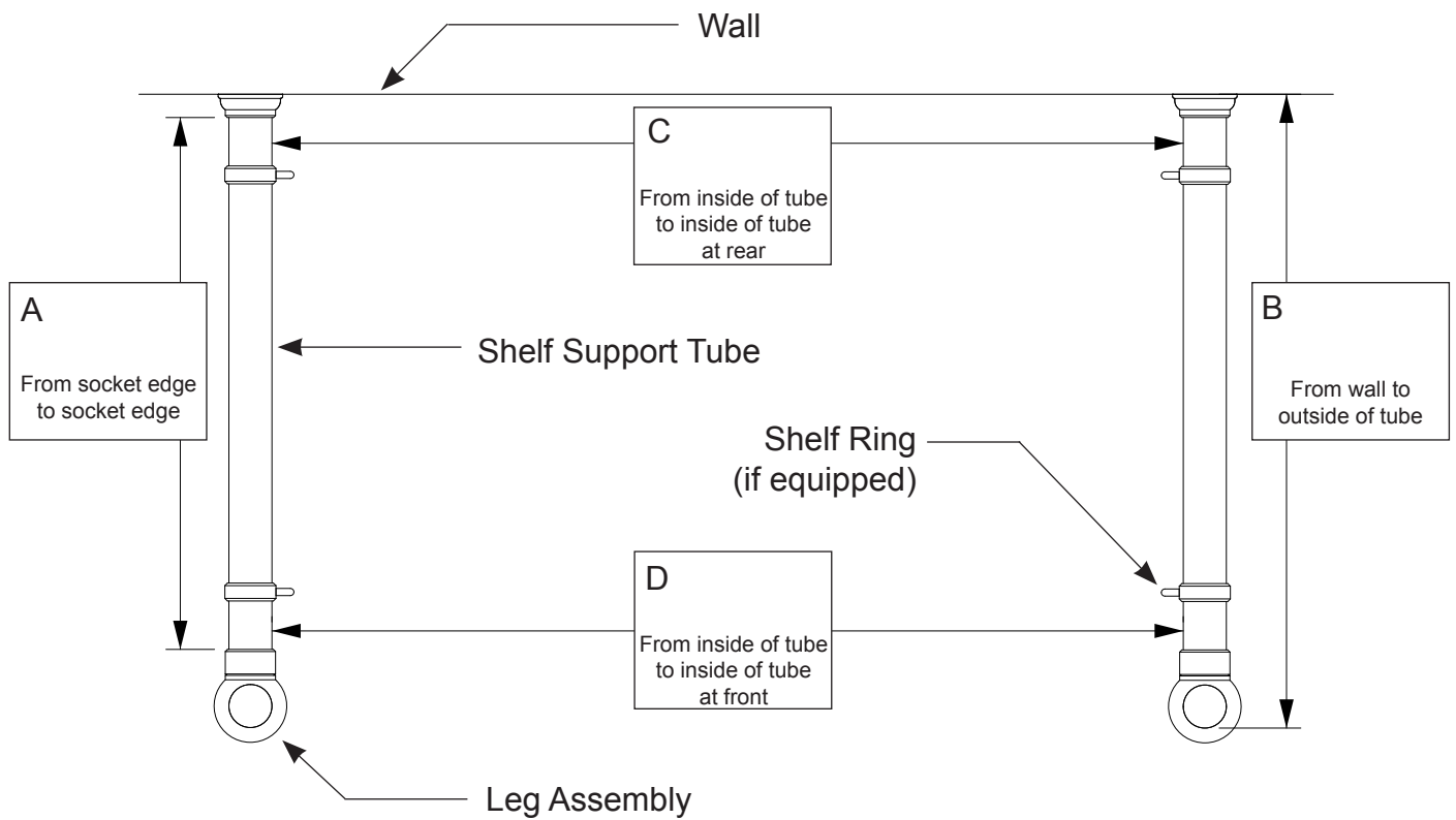
Plan View of Leg System at Shelf Support
